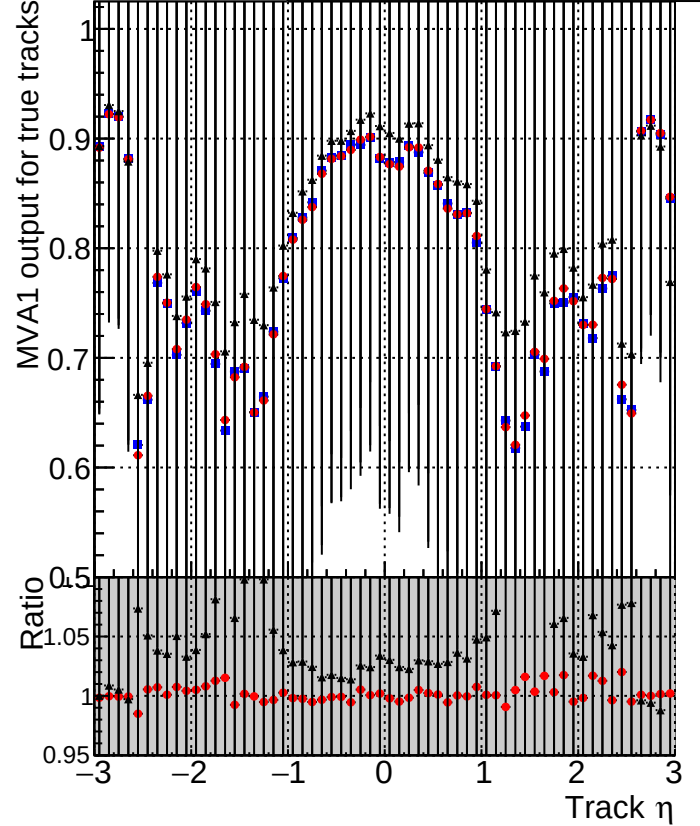
MVA1 of associated tracks (recoToSim) vs. track \eta Legend: DQM_mkFit_TT_baseR3_noSel_ok (blue squares) DQM_mkFit_TT_base_8iter_noSel_ok (red circles) DQM_mkFit_TT_Retrainv2_8iter_noSel_ok (black stars)
