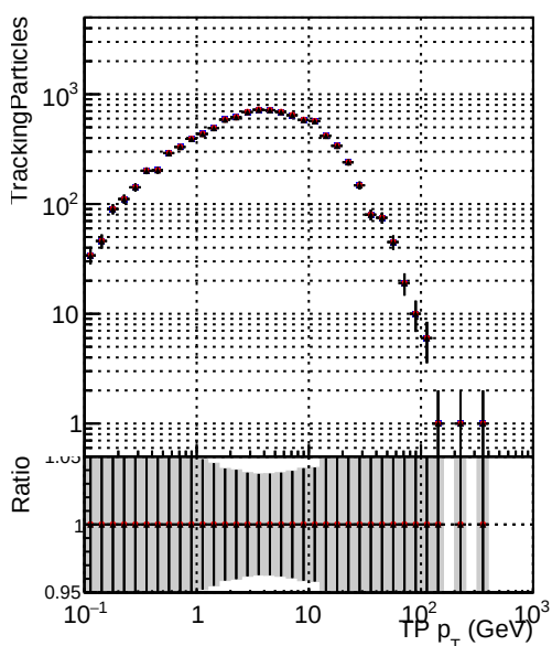
● DQM_mkFit_TT_baseR3_noSel_ok ● DQM_mkFit_TT_base_8iter_noSel_ok ● DQM_mkFit_TT_Retrainv2_8iter_noSel_ok
