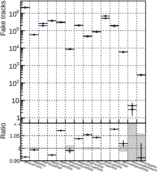
Number File 1 DQM_mkrFit_TT_base_8iter_noSel_ok 2 DQM_mkFit_TT_Retrainv2_8iter_noSel_ok
