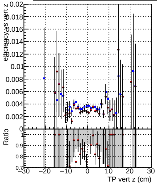
Efficiency vs. TP vert z — DQM_mkFit_TT_baseR3_noSel_ok — DQM_mkFit_TT_base_8iter_noSel_ok — DQM_mkFit_TT_Retrainv2_8iter_noSel_ok
