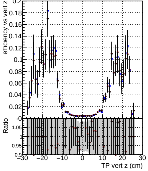
Efficiency vs. TP vert z (cm) — DQM_mkFit_TT_baseR3_noSel_ok — DQM_mkFit_TT_base_8iter_noSel_ok — DQM_mkFit_TT_Retrainv2_8iter_noSel_ok
