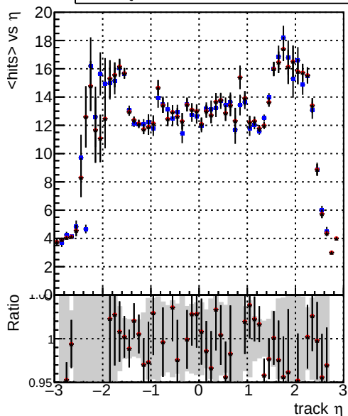
— DQM_mkFit_TT_baseR3_noSel_ok — DQM_mkFit_TT_base_8iter_noSel_ok — DQM_mkFit_TT_Retrainv2_8iter_noSel_ok
