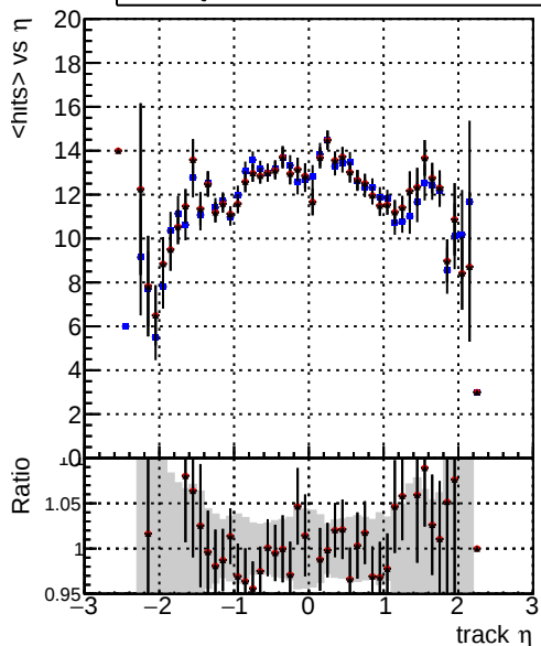
mean hit — DQM_mkFit_TT_baseR3_noSel_ok — DQM_mkFit_TT_base_8iter_noSel_ok — DQM_mkFit_TT_Retrainv2_8iter_noSel_ok
