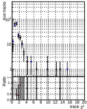
Ns of associated (recoToSim) tracks vs normalized \chi^2
