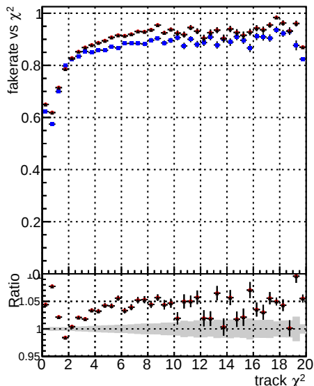
Fake rate vs. — DOM mkFit TT baseR3 noSel ok — DOM mkFit TT base 8iter noSel ok
