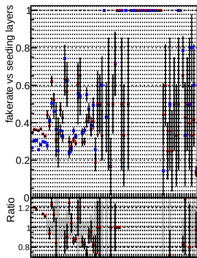
Fake rate vs. DOM mkFit TT baseR3 noSel ok DOM mkFit TT base 8iter noSel ok RetrainV2 8iter noSel ok
