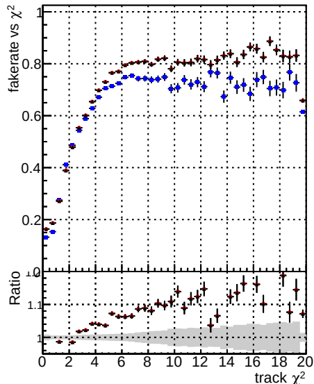
Fake rate vs. DOM mkFit TT baseR3 noSel ok DOM mkFit TT base 8iter noSel ok RetrainV2 8iter noSel ok
