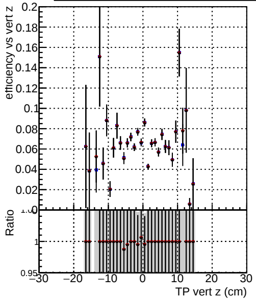
Efficiency vs vert z —●— DQM_mkFit_TT_baseR3_noSel_ok —●— DQM_mkFit_TT_base_8iter_noSel_ok —●— DQM_mkFit_TT_Retrainv2_8iter_noSel_ok
