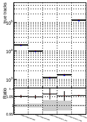
N of reco track vs. \chi^2 base after noSel ok DOM mkFit Retrainv2 after noSel ok
