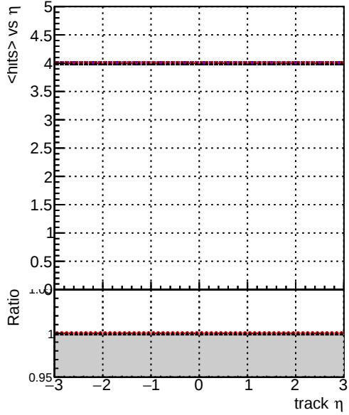
mean hits — DQM_mkFit_TT_baseR_noSel_ok — DQM_mkFit_TT_base_8iter_noSel_ok — DQM_mkFit_TT_Retrainv2_8iter_noSel_ok
