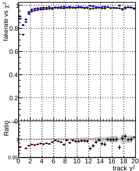
Fake rate vs. — DOM mkFit TT baseR noSel ok — DOM mkFit TT baseR noSel ok — DOM mkFit TT RetrainV2 8iter noSel ok
