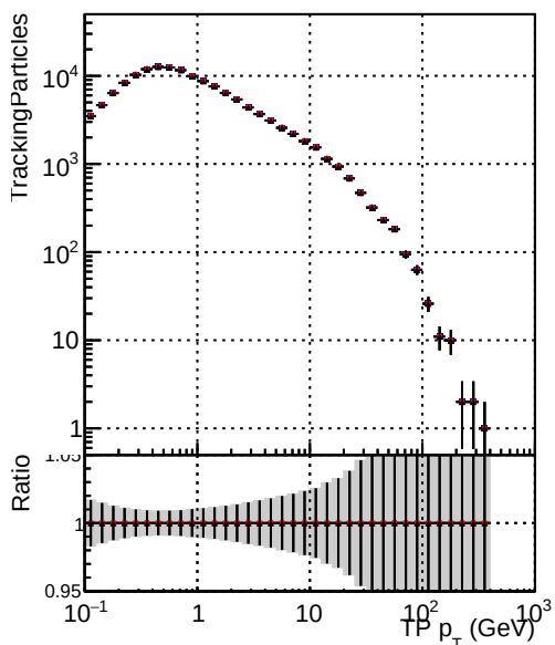
—•— DQM_mkFit_TT_baseR_noSel_ok —•— DQM_mkFit_TT_base_8iter_noSel_ok —•— DQM_mkFit_TT_Retrainv2_8iter_noSel_ok
