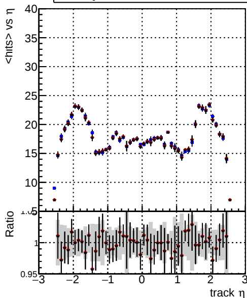
mean hits — DQM_mkFit_TT_baseR_noSel_ok — DQM_mkFit_TT_base_8iter_noSel_ok — DQM_mkFit_TT_Retrainv2_8iter_noSel_ok
