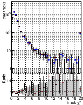
N of reco track vs. \chi^2 DGM mFit base noSel ok DGM mFit base after noSel ok DGM mFit Retrain2 after noSel ok
