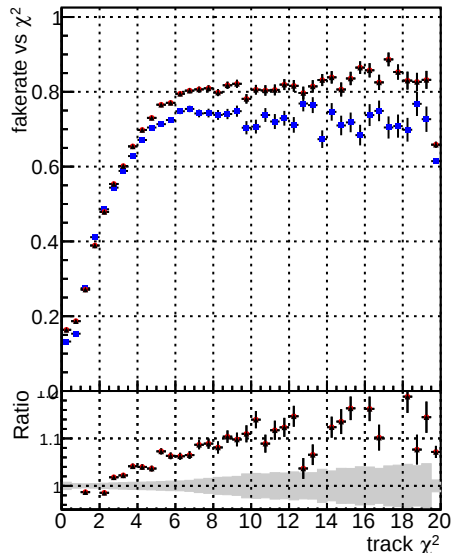
Fake rate vs. — DOM mkFit TT baseR noSel ok — DOM mkFit TT base 8iter noSel ok — RetrainV2 8iter noSel ok
