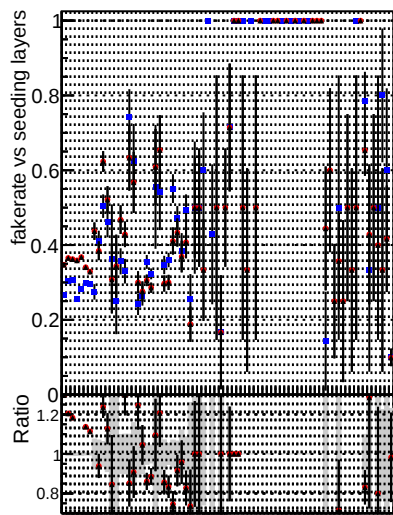
Fake rate vs. — DOM mkFit TT baseR noSel ok — DOM mkFit TT base 8iter noSel ok — RetrainV2 8iter noSel ok
