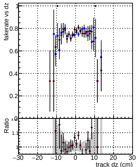
Fake rate vs dz Legend: DOM mkFit TT baseR noSel ok (blue) DOM mkFit TT base 3iter noSel ok (red) DOM mkFit TT RetrainV2 3iter noSel ok (black)
