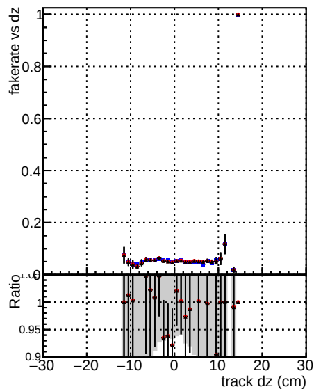
DOM mkFit TT baseR noSel ok DOM mkFit TT base 3iter noSel ok DOM mkFit TT RetrainV2 3iter noSel ok
