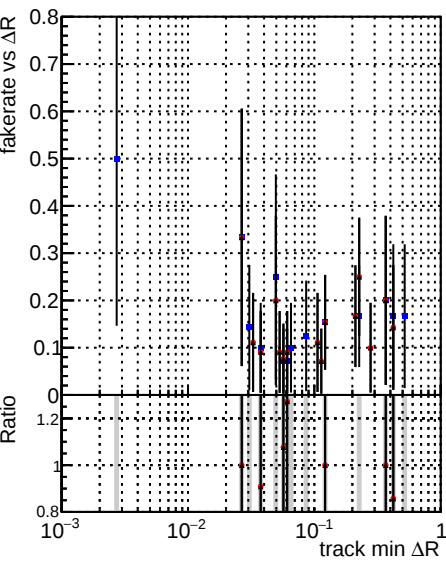
Legend: DQM_mkFit_TT_baseR_noSel_ok (blue dots), DQM_mkFit_TT_base_8iter_noSel_ok (red dots), DQM_mkFit_TT_Retrainv2_8iter_noSel_ok (black dots)
