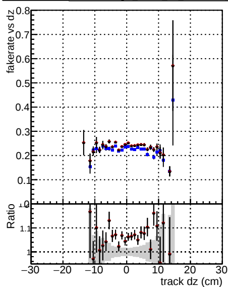
— DOM mkFit TT baseR noSel ok — DOM mkFit TT base 3iter noSel ok — DOM mkFit TT RetrainV2 3iter noSel ok
