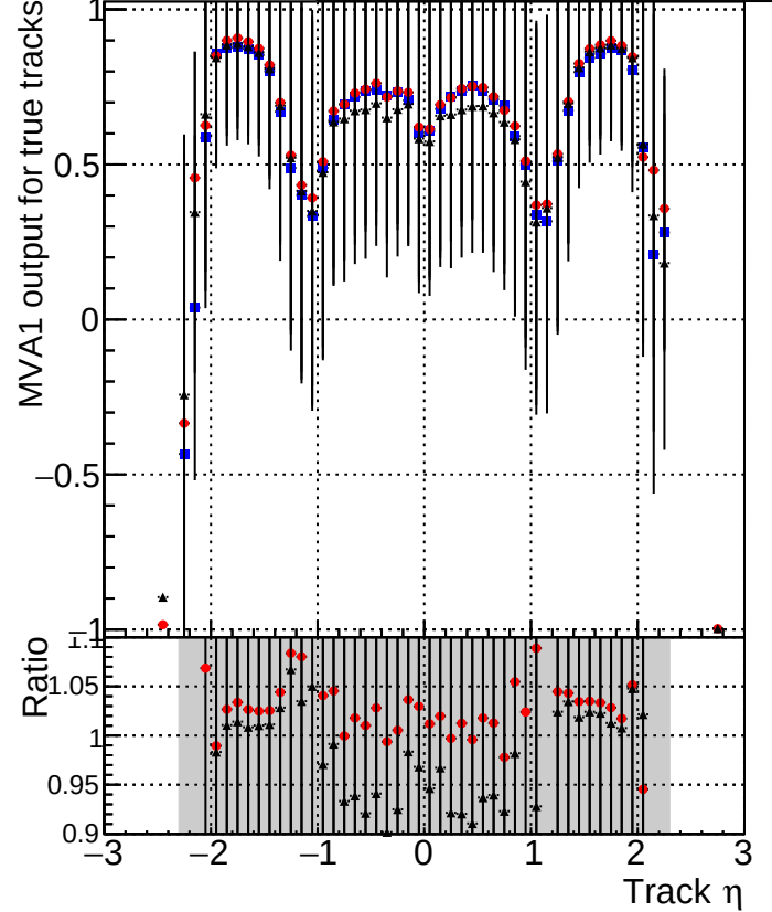
MVA1 of associated tracks (recoToSim) vs. track \eta Legend: DQM_mkFit_TT_baseR_noSel_ok (blue squares) DQM_mkFit_TT_base_8iter_noSel_ok (red circles) DQM_mkFit_TT_Retrainv2_8iter_noSel_ok (black triangles)
