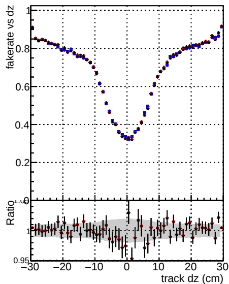
— DOM mkFit TT baseR noSel ok — DOM mkFit TT base 8iter noSel ok — DOM mkFit TT RetrainV2 8iter noSel ok
