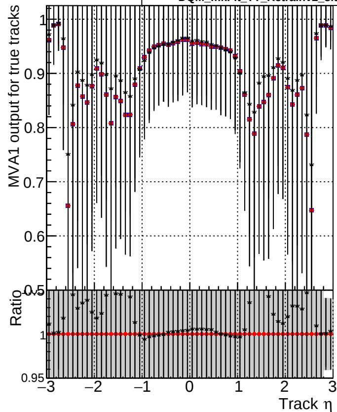
MVA1 of associated tracks (recoToSim) vs. track \eta Legend: ■ DQM_mkFit_TT_baseR_noSel_ok ● DQM_mkFit_TT_base_8iter_noSel_ok ▲ DQM_mkFit_TT_Retrainv2_8iter_noSel_ok
