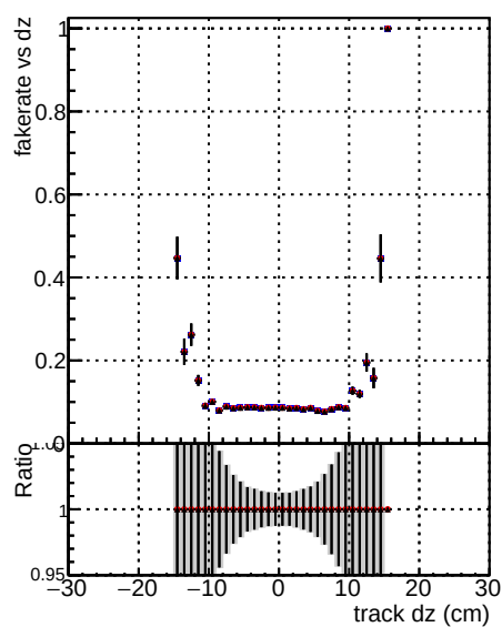
Fake rate vs dz DQM mkFit TT baseR noSel ok DQM mkFit TT base 3iter noSel ok DQM mkFit TT RetrainV2 8iter noSel ok
