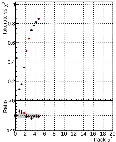
Fake rate vs. DOM mkFit TT baseR noSel ok DOM mkFit TT base 8iter noSel DOM mkFit TT RetrainV2 8iter noSel
