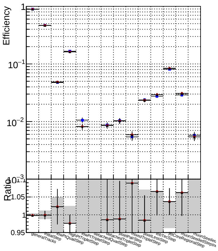
DQM_mkFit_TT_baseR_noSel_ok DQM_mkFit_TT_base_8iter_noSel_ok DQM_mkFit_TT_Retrainv2_8iter_noSel_ok
