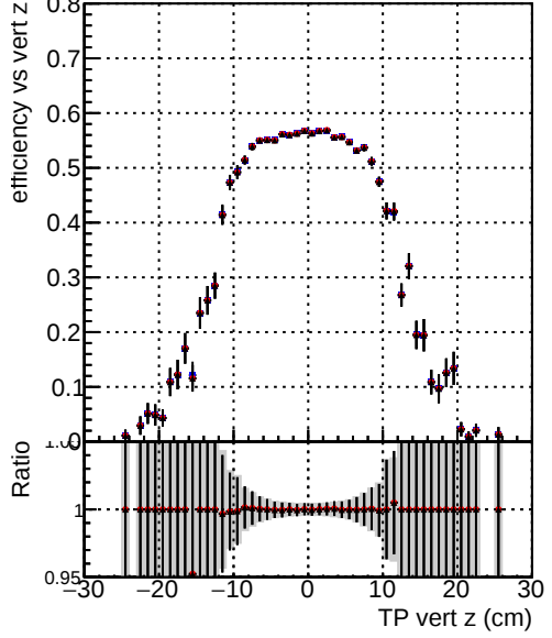
Efficiency vs. sim PV z — DQM_mkFit_TT_baseR_noSel_ok — DQM_mkFit_TT_base_8iter_noSel_ok — DQM_mkFit_TT_Retrainv2_8iter_noSel_ok
