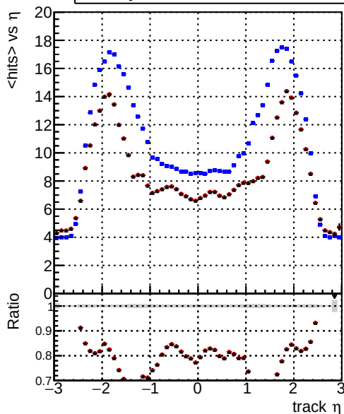
— DQM_mkFit_TT_baseR_noSel_ok — DQM_mkFit_TT_base_8iter_noSel_ok — DQM_mkFit_TT_Retrainv2_8iter_noSel_ok mean hits
