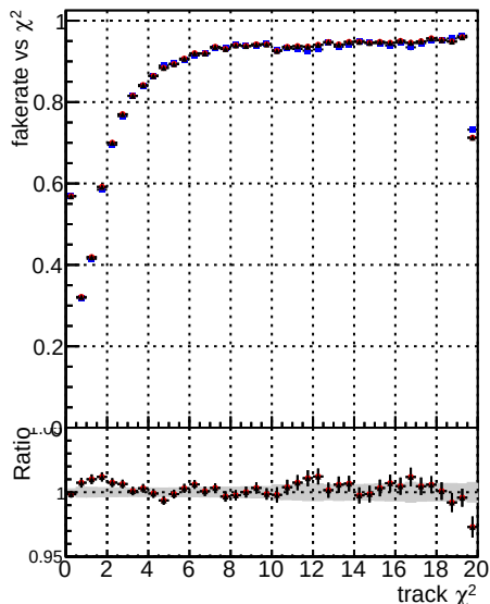
Fake rate vs. DOM mkFit TT baseR noSel ok DOM mkFit TT base 8iter noSel ok DOM mkFit TT RetrainV2 8iter noSel ok
