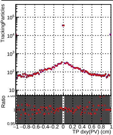
N of sim DQM_CKF_TT_retrainOldFiles125_v2_prelimWP3_epoch4
