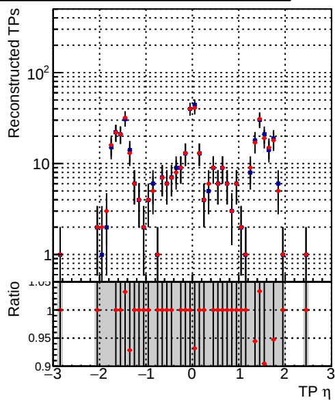
N of simulated tracks vs \eta —•— DQM_CKF_TTbase —•— DQM_CKF_TT_retrainOldFiles125_v2_prelimWP3_epoch4
