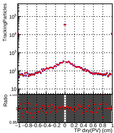
N of sim DQM_CKF_TT_retrainOldFiles125_v2_prelimWP3_epoch4
