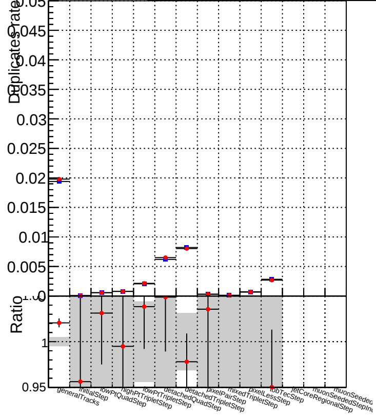
Duplicates rate vs collection Legend: DQM_CKF_TTbase (blue square) DQM_CKF_TT_retrainOldFiles125_v2_prelimWP3_epoch4 (red circle)
