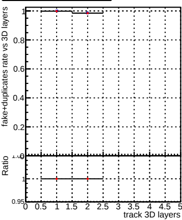
fake+duplicates rate vs 3D layers
