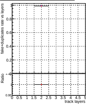
fake+duplicates rate vs layers
