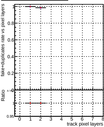
fake+duplicates rate vs pixel layers
