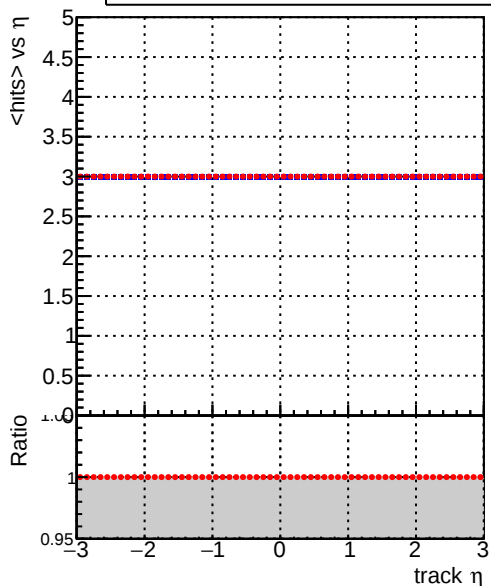
mean hits vs \eta Legend: DQM_CKF_TTbase (blue line), DQM_CKF_TT_retrainOldFiles125_v2_prelimWP3_epoch4 (red line)
