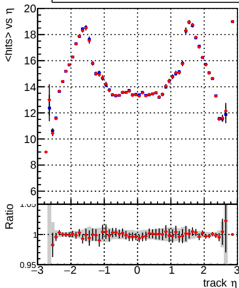
mean hits vs \eta — DQM_CKF_TTbase — DQM_CKF_TT_retrainOldFiles125_v2_prelimWP3_epoch4
