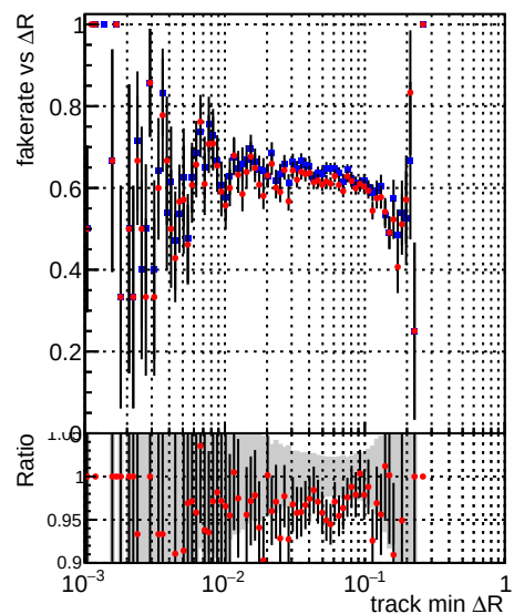
— DQM_CKF_TTbase — DQM_CKF_TT_retrainOldFiles125_v2_prelimWP3_epoch4
