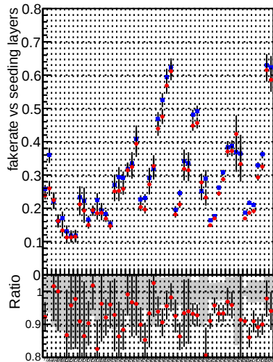
Fake rate vs. —♦— DQM_CKF_TTbase —★— DQM_CKF_TT_retrainOldFiles125_v2_prelimWP3_epoch4
