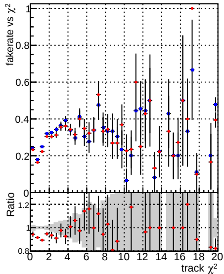
Fake rate vs. —♦— DQM_CKF_TTbase —★— DQM_CKF_TT_retrainOldFiles125_v2_prelimWP3_epoch4
