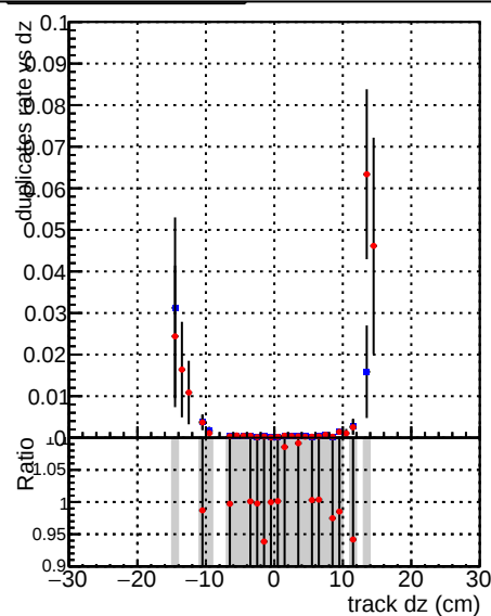
—●— DQM_CKF_TTbase —●— DQM_CKF_TT_retrainOldFiles125_v2_prelimWP3_epoch4
