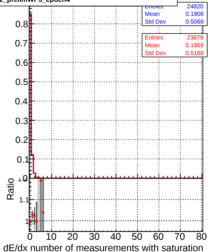
■ DQM_CKF_TTbase ● DQM_CKF_TT_retrainOldFiles125_v2_prelimWP3_epoch4
