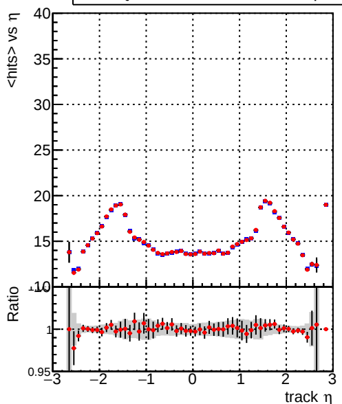
mean hits vs \eta Legend: DQM_CKF_TTbase (blue line), DQM_CKF_TT_retrainOldFiles125_v2_prelimWP3_epoch4 (red line)
