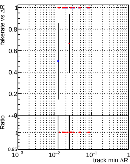
Legend: DQM_CKF_TTbase (grey bars), DQM_CKF_TT_retrainOldFiles125_v2_prelimWP3_epoch4 (red dots with error bars)
