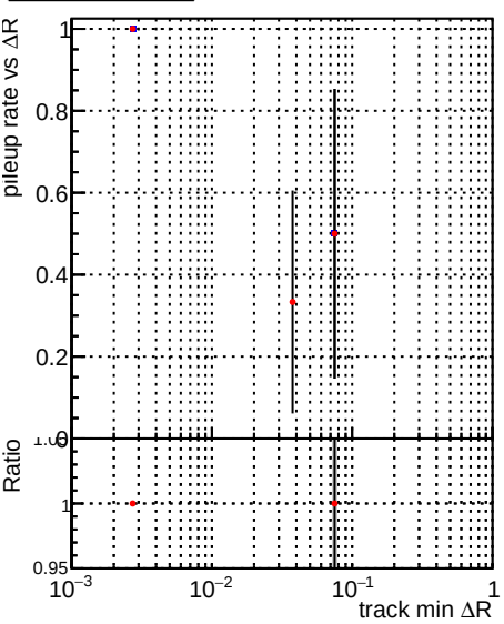
Legend: DQM_CKF_TTbase (blue dots), DQM_CKF_TT_retrainOldFiles125_v2_prelimWP3_epoch4 (red dots)
