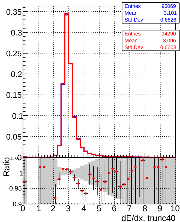
—■— DQM_CKF_TTbase —●— DQM_CKF_TT_retrainOldFiles125_v2_prelimWP3_epoch4
