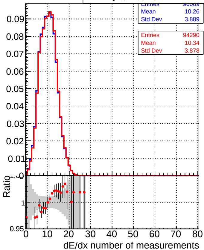
—■— DQM_CKF_TTbase —●— DQM_CKF_TT_retrainOldFiles125_v2_prelimWP3_epoch4
