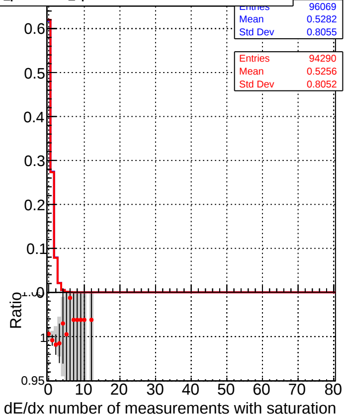
—■— DQM_CKF_TTbase —●— DQM_CKF_TT_retrainOldFiles125_v2_prelimWP3_epoch4
