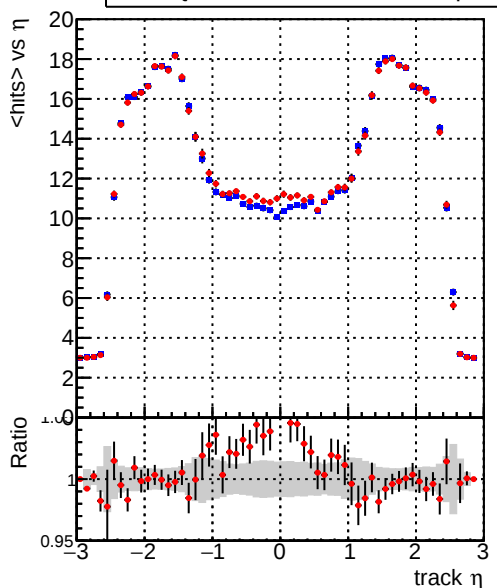
— DQM_CKF_TTbase — DQM_CKF_TT_retrainOldFiles125_v2_prelimWP3_epoch4
