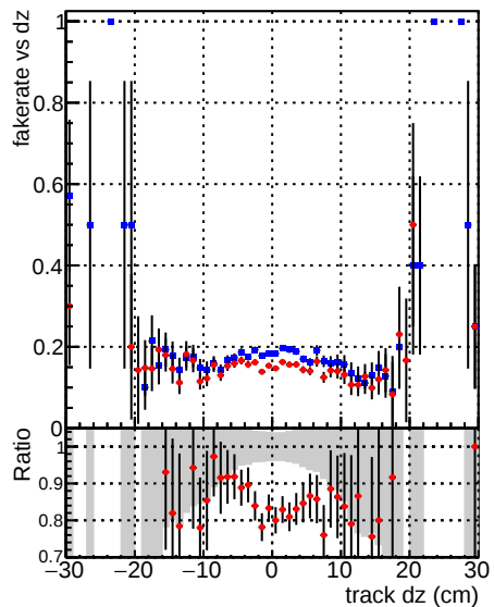
—●— DQM_CKF_TTbase —●— DQM_CKF_TT_retrainOldFiles125_v2_prelimWP3_epoch4
