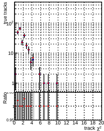
N of reco track vs. \chi^2 for DQM_CKF_TTbase and DQM_CKF_TT_retrainOldFiles125_v2_prelimWP3_epoch4
