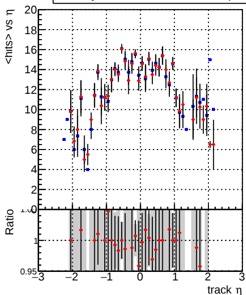
mean hits vs \eta Legend: DQM_CKF_TTbase (blue line with markers), DQM_CKF_TT_retrainOldFiles125_v2_prelimWP3_epoch4 (red line with markers)
